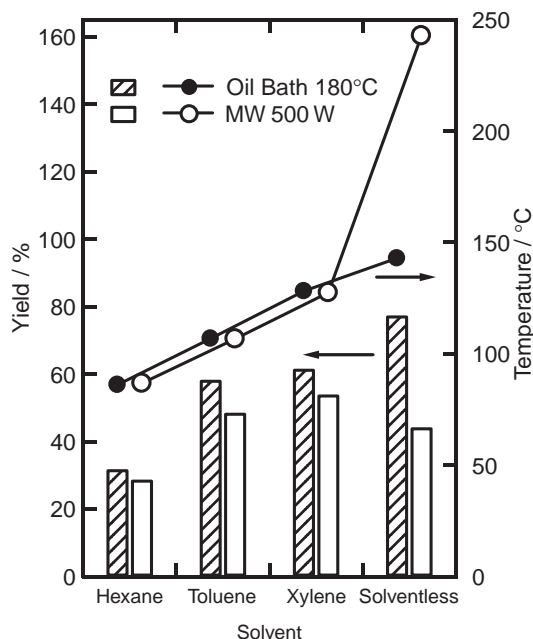
Figure 2. The yields of 4-methyl-2,3-dihydro-1H-1,5-benzodiazepin-2-one by the reaction of 1,2-phenylenediamine and ethyl acetoacetate and the temperatures just after the reactions in different solvents. The heating times are 10 min.
