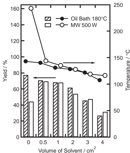
Figure 3. The yield of 4-methyl-2,3-dihydro-1H-1,5-benzodiazepin-2-one by the reaction of 1,2-phenylenediamine and ethyl acetoacetate and the temperatures just after the reactions in different volume of the solvent of xylene. The heating times are 10 min.
