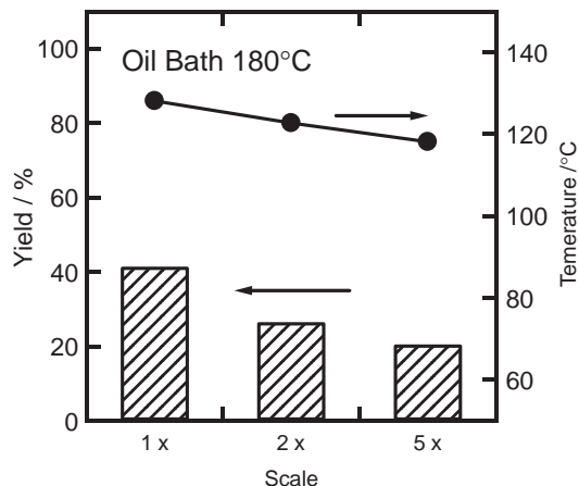
Figure 4. The yields of 4-methyl-2,3-dihydro-1H-1,5-benzodiazepin-2-one by the reaction of 1,2-phenylenediamine and ethyl acetoacetate and the temperatures just after the reaction in different scales. The heating times are 2 min.
